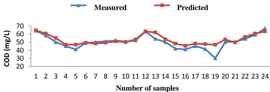
Figure 1b: The comparison between COD values calculated by the regression equation and actual values measured in samples
