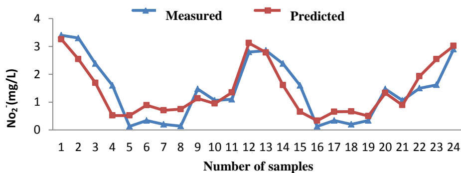
Figure 3: The comparison between \text{NO}_2 values calculated by the regression equation and actual values measured in samples
