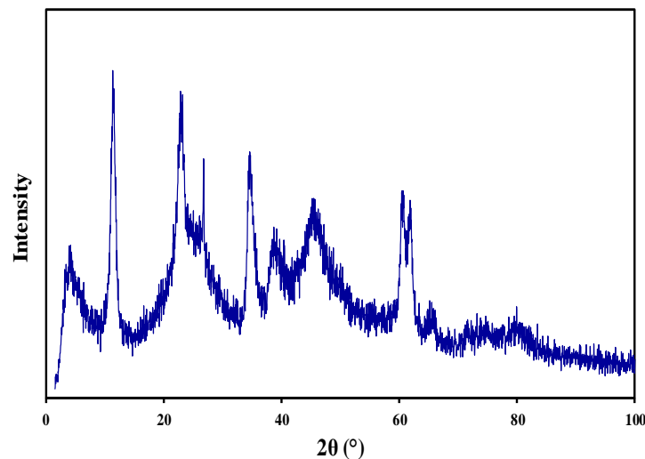
Figure 2: The XRD pattern of Mg-Al-LDH
