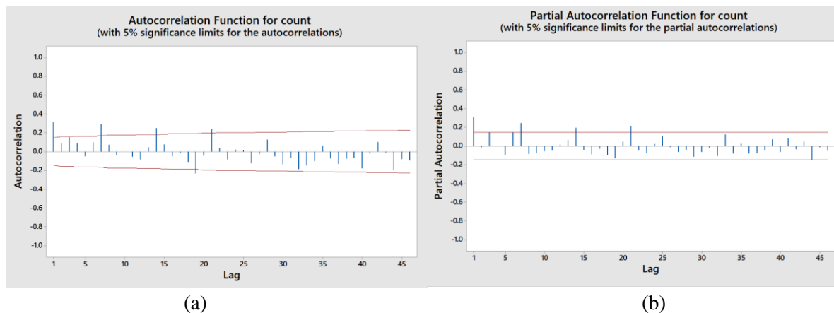
Figure 4: ACF Plot (a) and PACF Plot (b)
