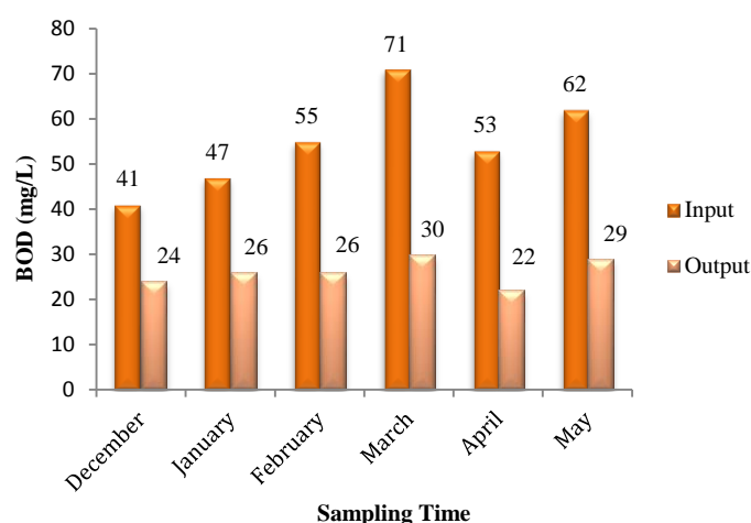
Figure 1: The trend of changes in \text{BOD}_5 in the input and output wastewater treatment plant
