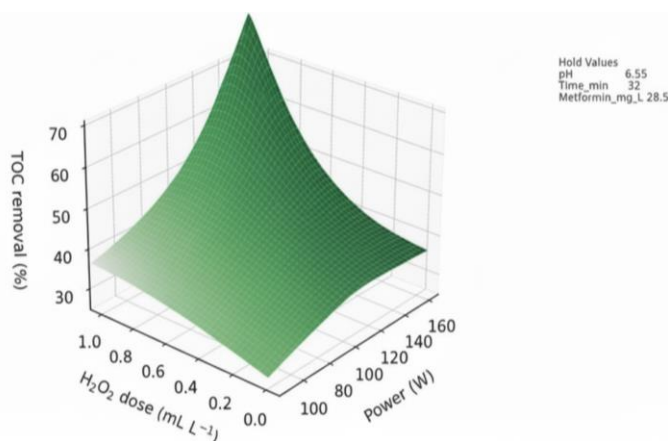
Figure 11: 3D Surface Plot: Effect of Ultrasonic Power and H 2 O 2 Dose on TOC Removal.
