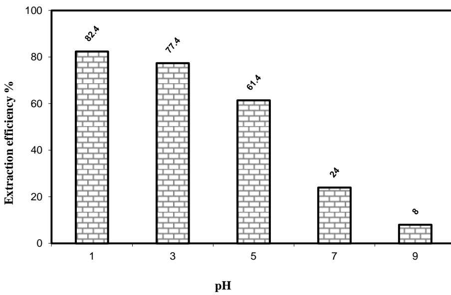
Figure 3: Efficiency of XAD-7HP resin in various pH (humic acid concentration of 5 mg/L and constant for all samples)
