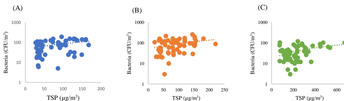
Figure 1: The association between TSP and bacterial concentration. (A) Medical ward, (B) Infectious diseases ward, (C) Outdoor air
