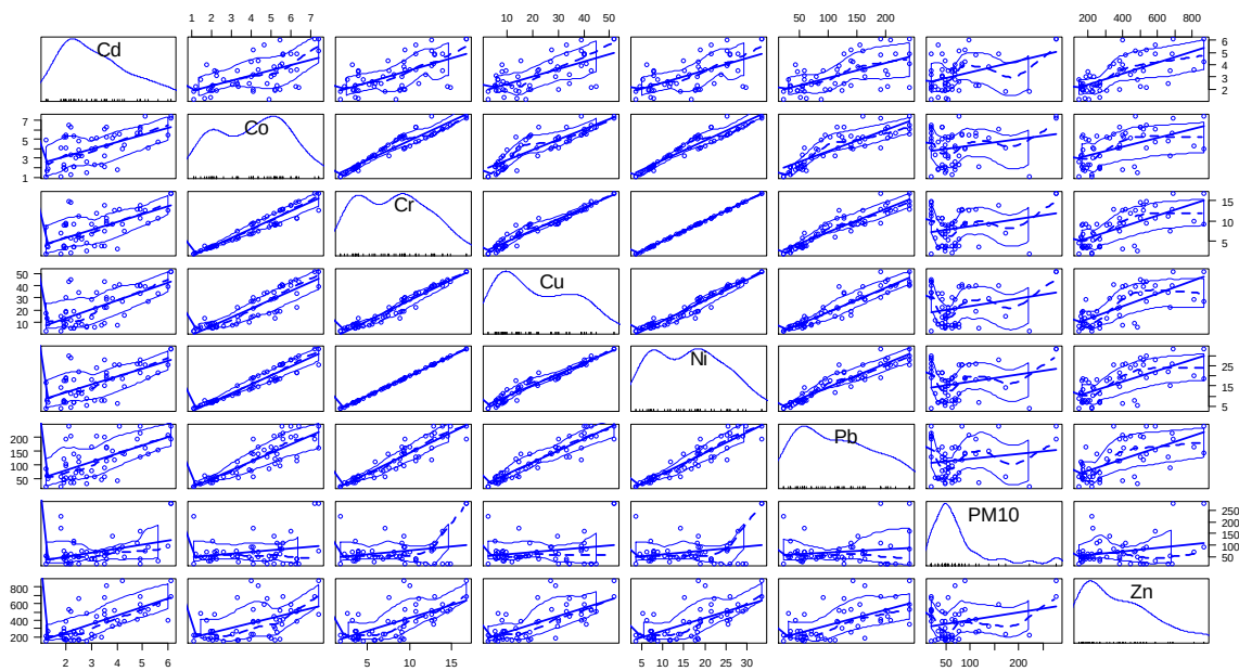
Figure 2: Graphical representation of correlation patterns between PM 10 and heavy metals.
